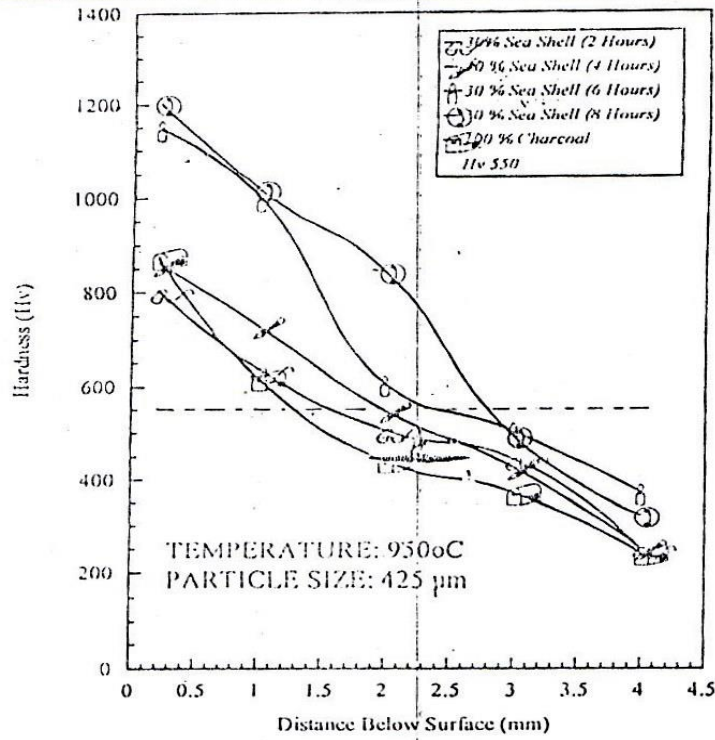
Figure 2: Effect of Holding Time on the Carburizing Kinetics Using 30 % Sea Shell at 950 oC
