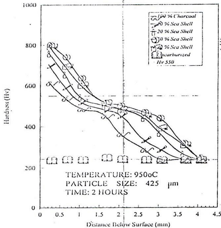
Figure 1: Graphical - Determination of Case Depth using Hardness Profiles and distance data for Different Carburizing Compounds after 2 Hours at 950 oC
